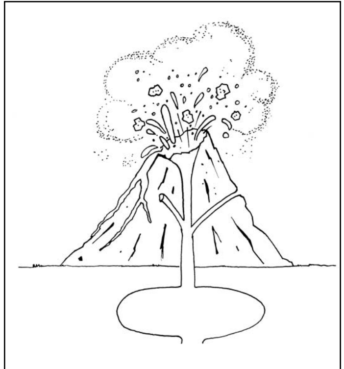
rock fragments
