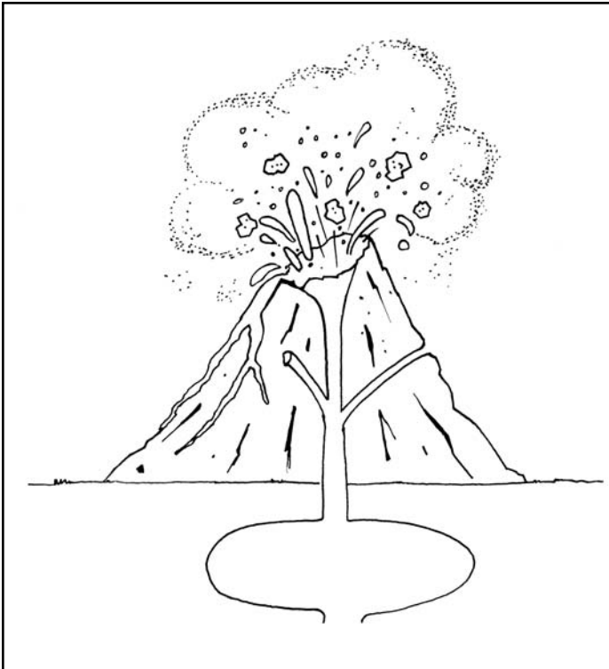
volcano
